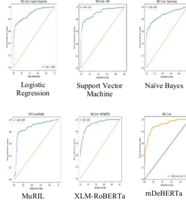
Figure 8 : ROC curves
