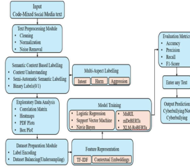
Figure 5-Model Architecture
